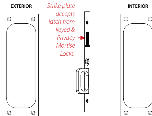
Dummy Door Mortise Lock
