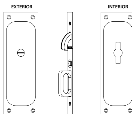
Privacy Door Mortise Lock
