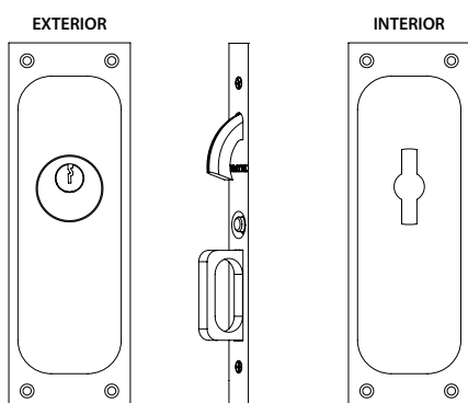
Keyed Door Mortise Lock
